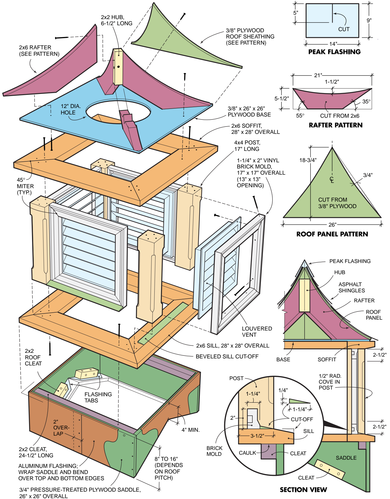
Fig. A Cupola Details
